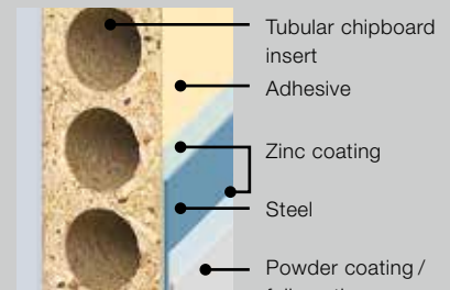
Tubular chipboard insert (Standard)
