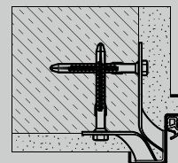
Fitting with through plugs (Plug-and-screw fitting)
