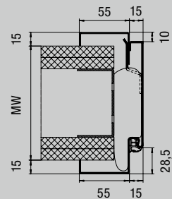
Profile 31103, rebated
