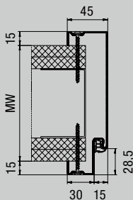
Profile 21120, screw fixing through frame face
