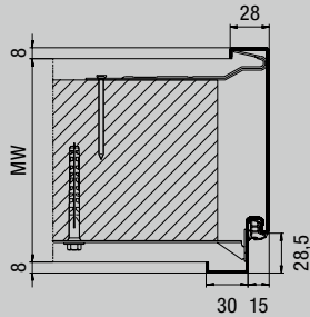
Profile 21100
