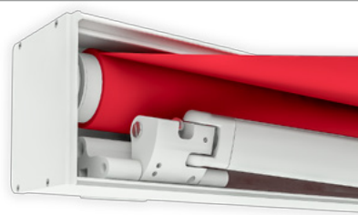
the windlock mechanism prevents the awning from lifting up at the front in windy conditions
