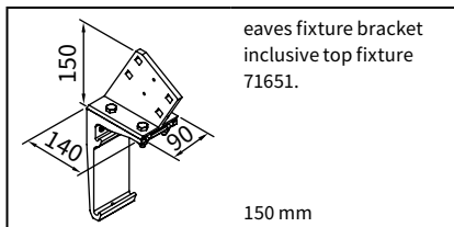
flat plate and angled bracket for eaves fixture
