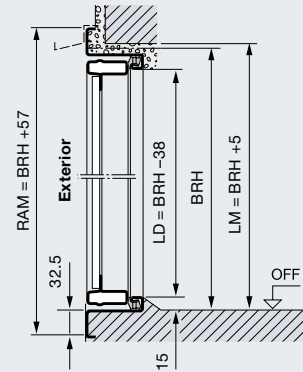
Single-leaf with threshold (the threshold is removed on-site)
