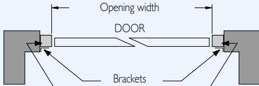
Fitting to Quick-fit steel Retractable frame, within the brickwork aperture
