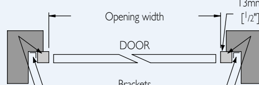
Fitting to Quick-fit steel Retractable frame, behind the brickwork aperture
