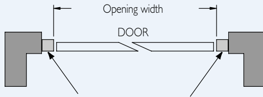
70mm x 70mm [2 3/4" x 2 3/4"] timber frame to be supplied and fixed by the customer
