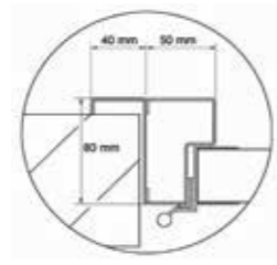
Frame dimensions.
